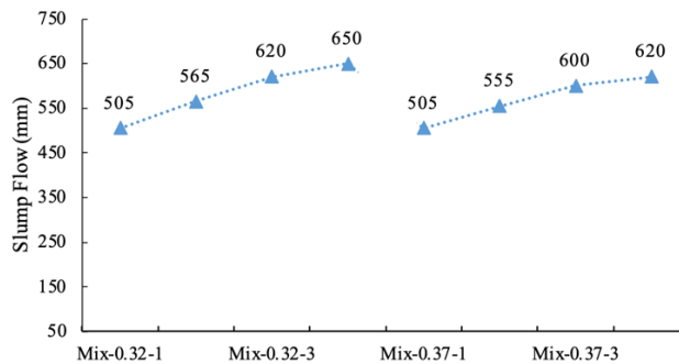
Fig. 2. Slump flow test results of the concrete mixtures for w/b ratios 0.32 and 0.37.
