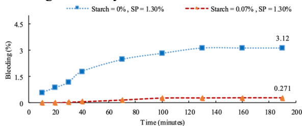
Fig. 5. Bleeding test results of the SCC mixtures with and without starch.
