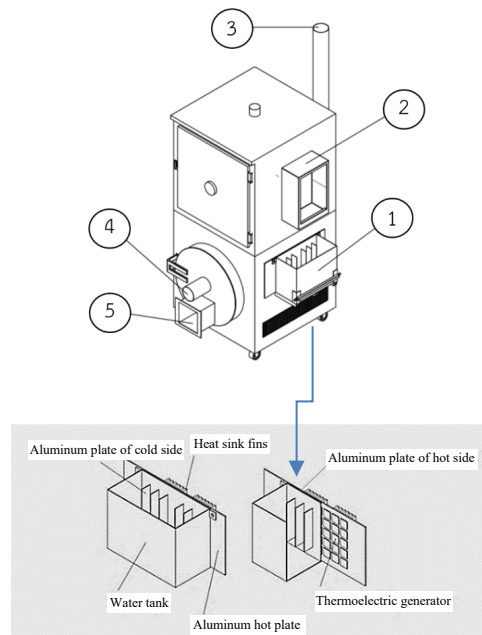
Fig. 3. Hybrid circuit for generating electricity from thermoelectric modules.
