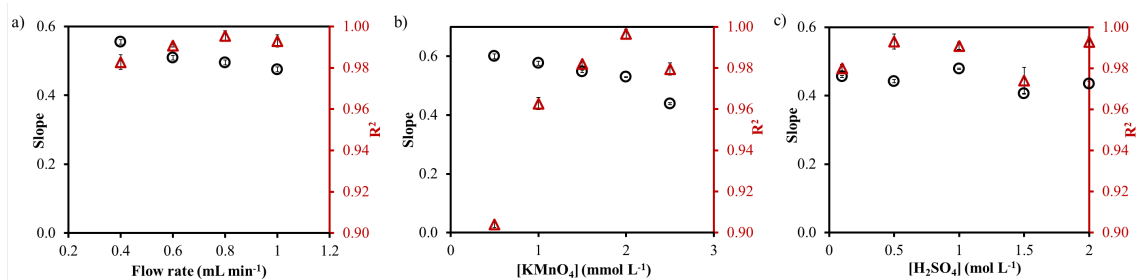
Fig. 7. The optimization study of 3D LOC coupled with r-FIA system for determination of cinnarizine, a) Effect of flow rate (mL min -1 ); b) [KMnO 4 ] (mmol L -1 ); and c) [H 2 SO 4 ] (mol L -1 ) in the system.
