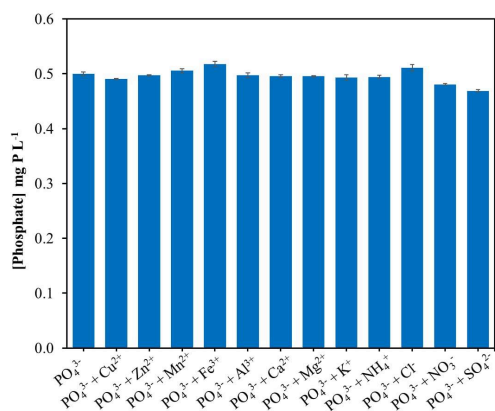
Fig. 4. Effect of interferences on phosphate determination.
