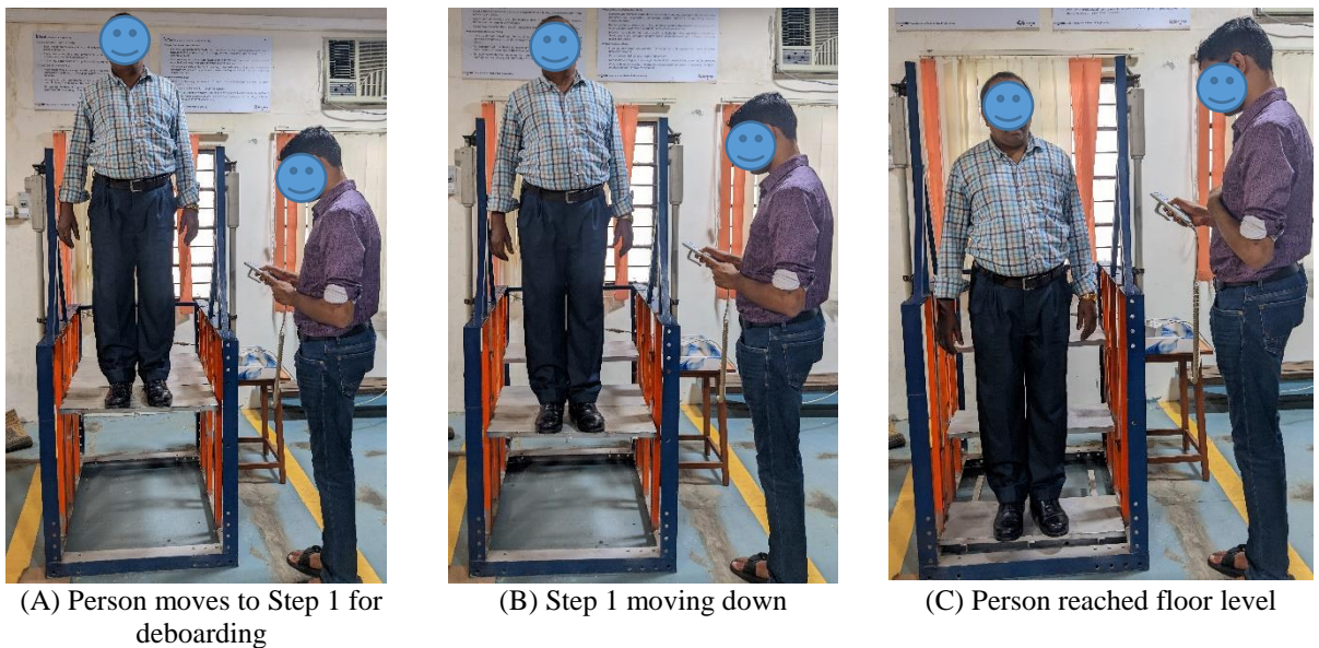
Fig. 17. Laboratory Trials of dynamic steps when deboarding
