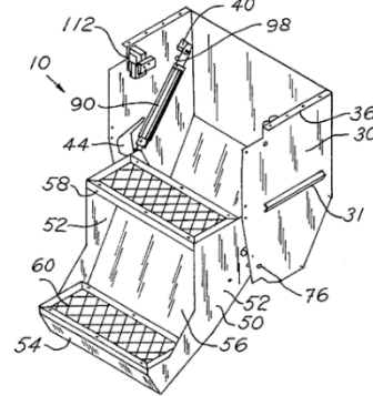
Fig. 4. Folding system for Vehicles [26]
