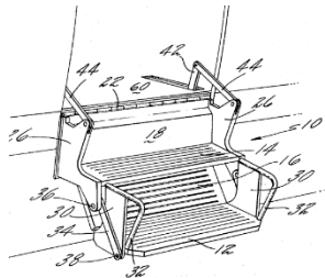
Fig. 1. Folding staircase [23]
