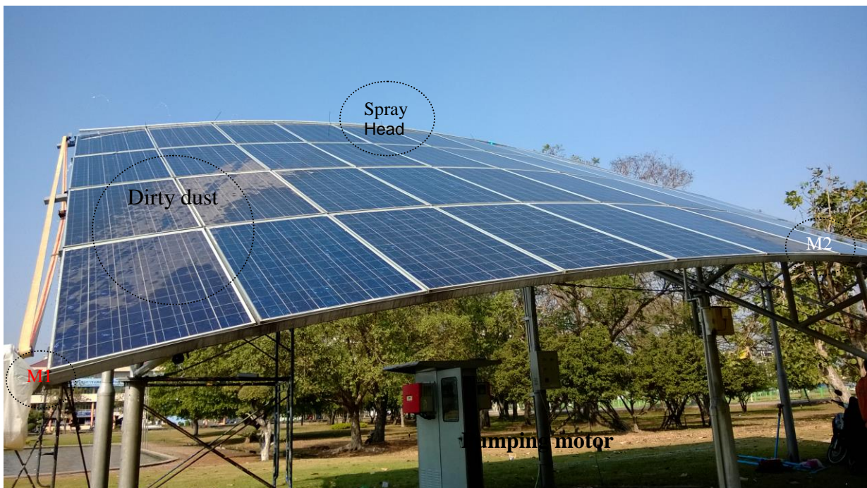
Figure 6: The smallest dirty dust on PV panels.
