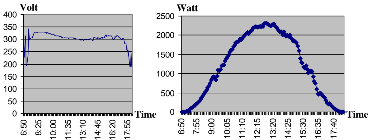
Figure 1: Voltage and Power of the 10 kW system.
