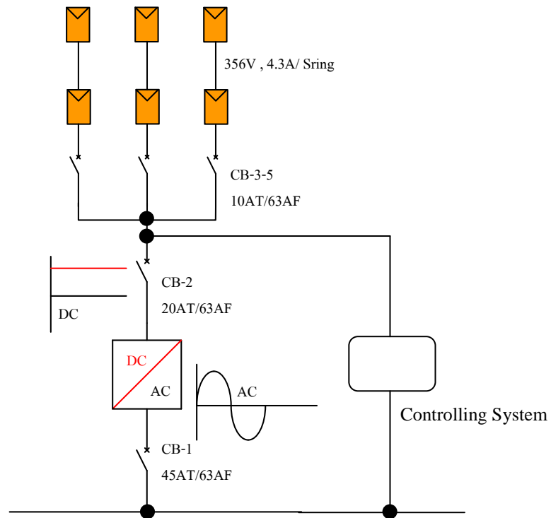
Figure 2: single line diagram of 10 kWp photovoltaic system.
