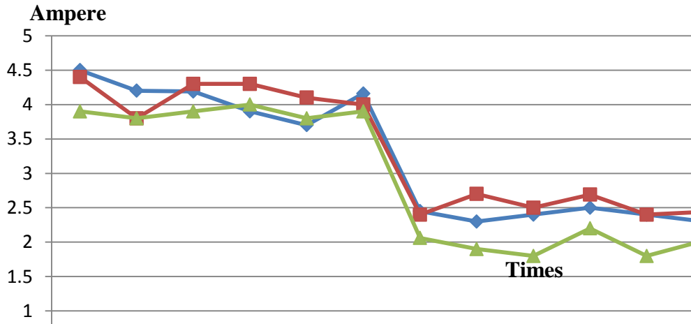
Figure 9: Output current of the single phase inverter.
