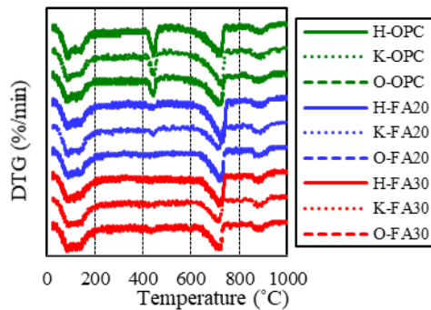
Figure 6. Results of DTG analysis.
