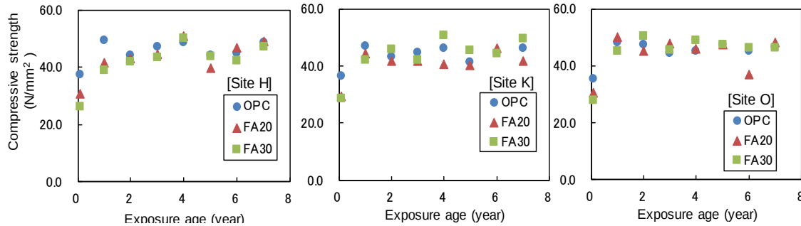
Figure 2. Changes in compressive strength with exposure age.
