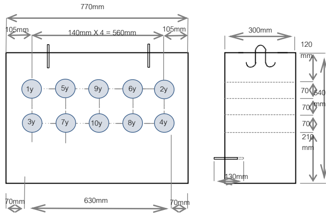
Figure 1. Outline of Exposed specimen.
