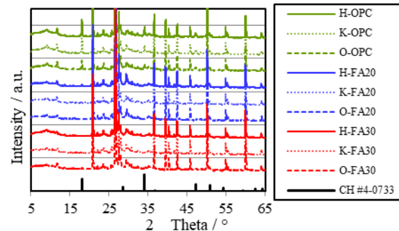
Figure 7. Results of XRD analysis.
