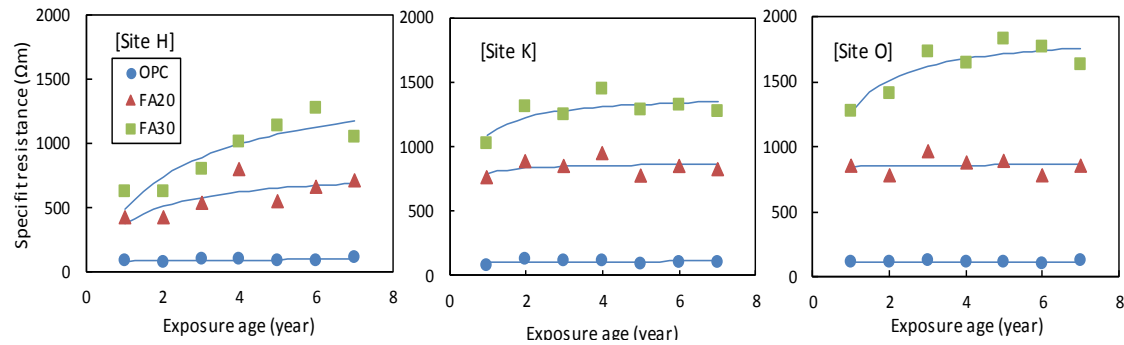
Figure 3. Changes in volume resistivity with exposure age.
