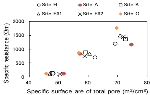
Figure 4. The relationship between the Specific surface area of total pore and volume resistivity.
