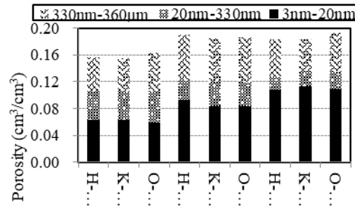
Figure 5. Pore size distribution.
