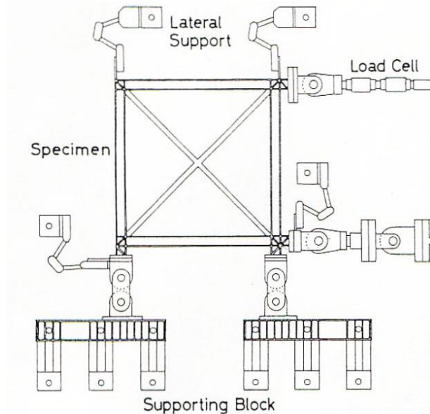
Figure 1. Brace Configuration on the testing Assembly (Wakabayashi et al. 1980).
