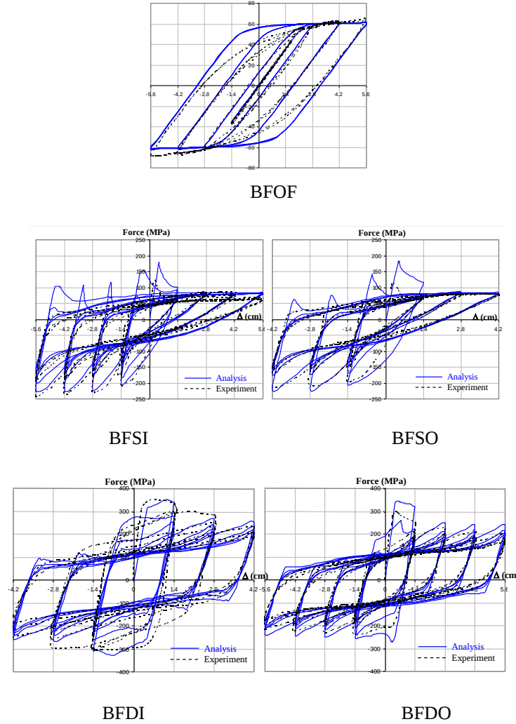
Figure 3. Lateral force-displacement at top of the frames.
