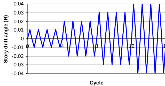
Figure 2. Loading pattern.
