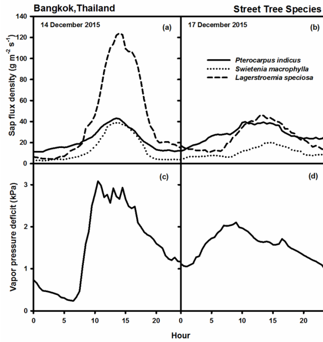
Figure 1: Diurnal patterns of sap flux density of all species during a high (a) and low (b) atmospheric demand days. Variation of vapor pressure deficit during a 24-hour period (c and d).
