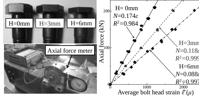
(a) Specimen and test situation. (b) Measurement result.
