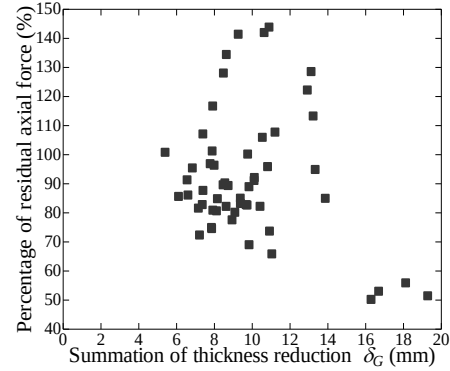
Figure 5. Relationship between residual axial force and thickness reduction.
