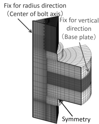
Figure 9. Analysis model.
