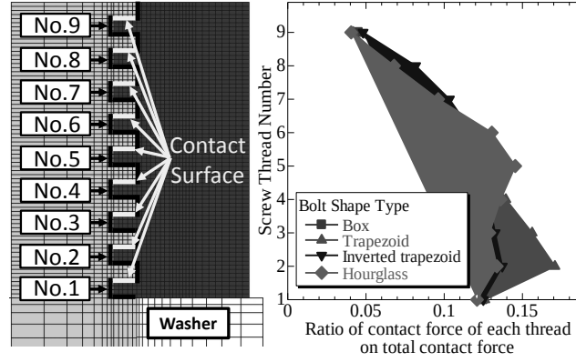
Figure 12. Ratio of contact force of each screw thread.
