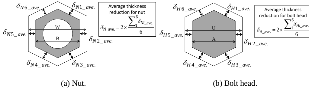
Figure 3. Definition of average thickness reduction.
