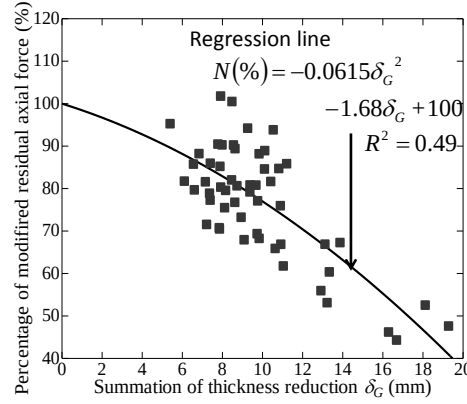
Figure 7. Relationship between residual axial force and thickness reduction.
