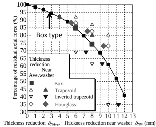
Figure 11. Analysis results.
