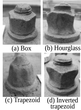
Figure 8. Examples of corroded bolt shape.
