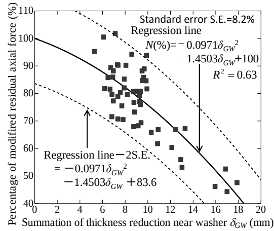
Figure 13. Reevaluated test results of residual axial force and thickness reduction near washer.
