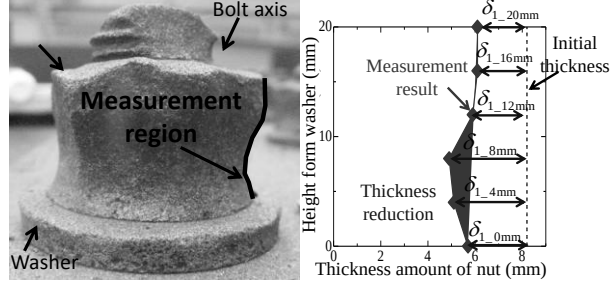
Figure 2. Example of measurement results of bolt shape.
